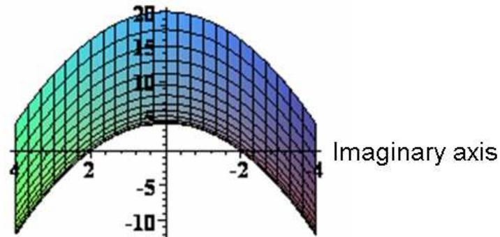
Purely imaginary number axis
