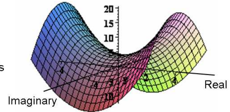
Both axes shown
